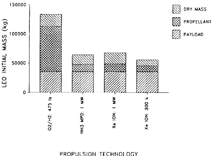
Fig. 1. Propulsion system mass comparison.
