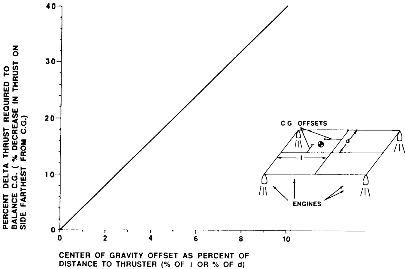
Fig. 10. Throttability required to balance center-of-gravity offsets.
