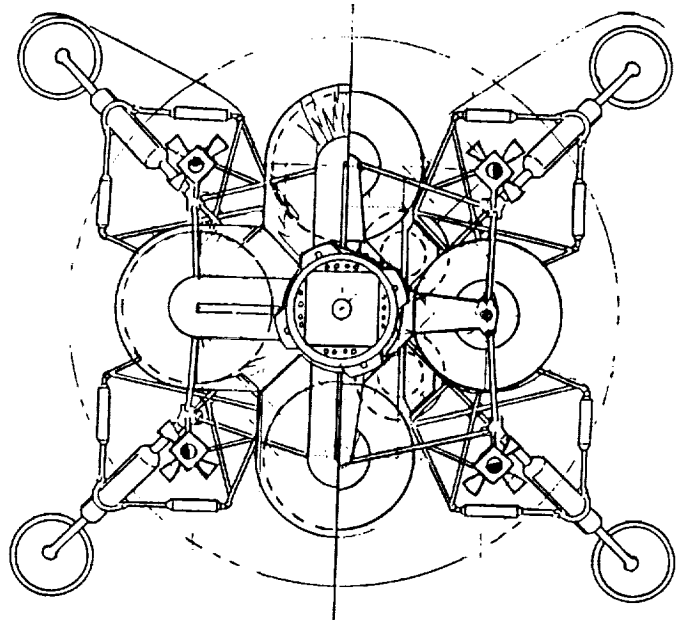
Fig. 10. Advanced reusable lunar lander, top view.
