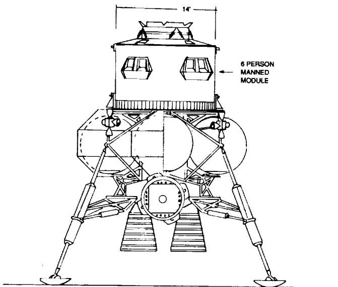
Fig. 9. Advanced reusable lunar lander, side view.
