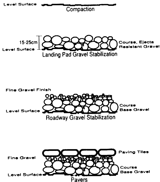
Fig. 7. Surface stabilization.
