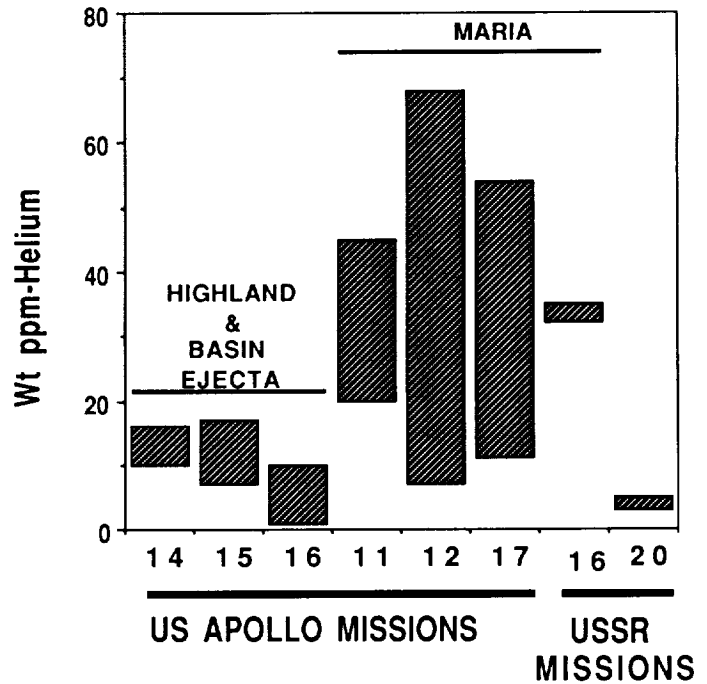
Fig. 10. Measured He content in lunar samples.
